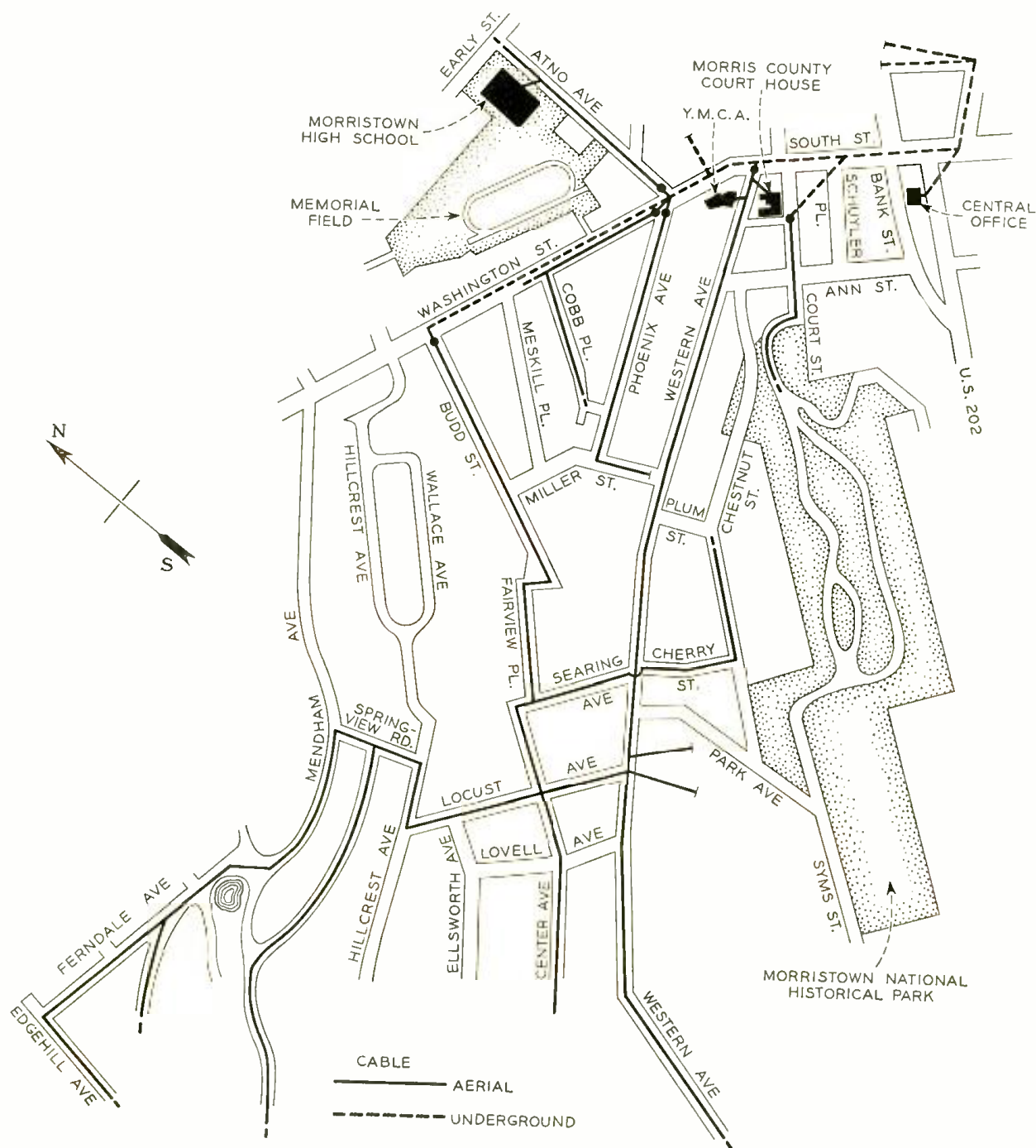
Fig. 6—At Morristown, New Jersey, this exchange area cable system was tested for advantages of gas pressure as an economical means of keeping out moisture and detecting sheath leakage. Successful results led to more extensive tests now in progress in Caldwell, New Jersey. Formerly only toll cable was pressurized.
