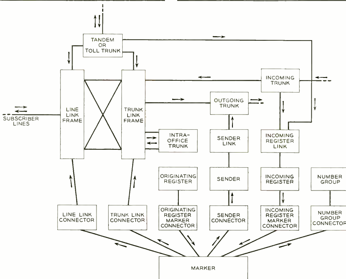
Fig. 6—Block diagram showing circuits required for a completing call.
