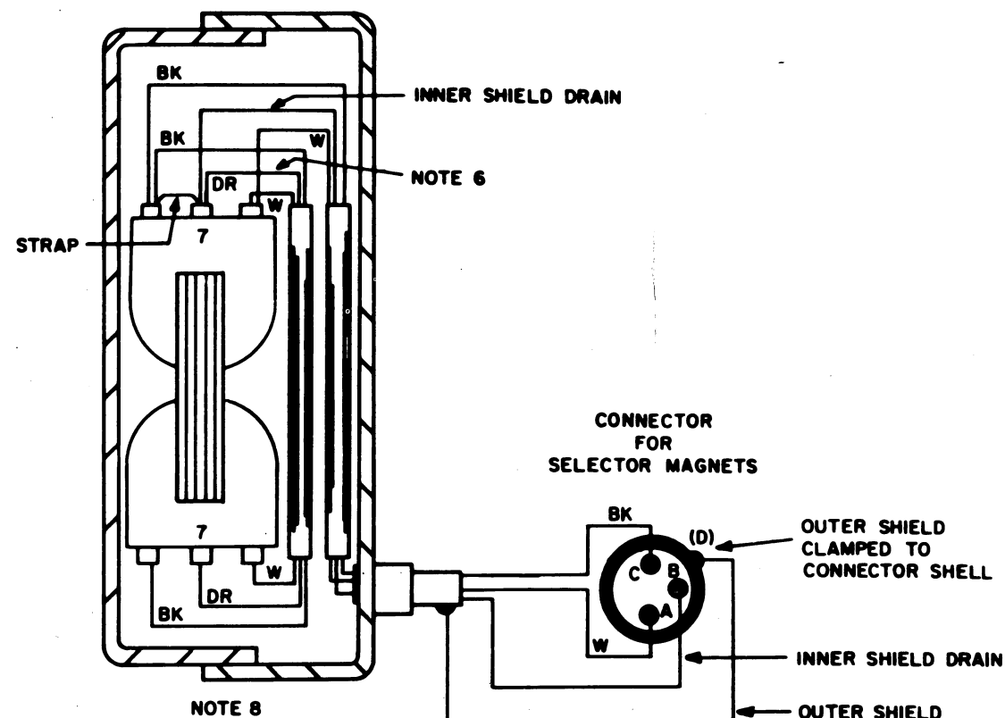
A SELECTOR MAGNETS
