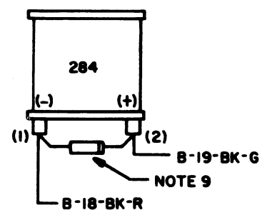
D BACKSPACE MAGNET
