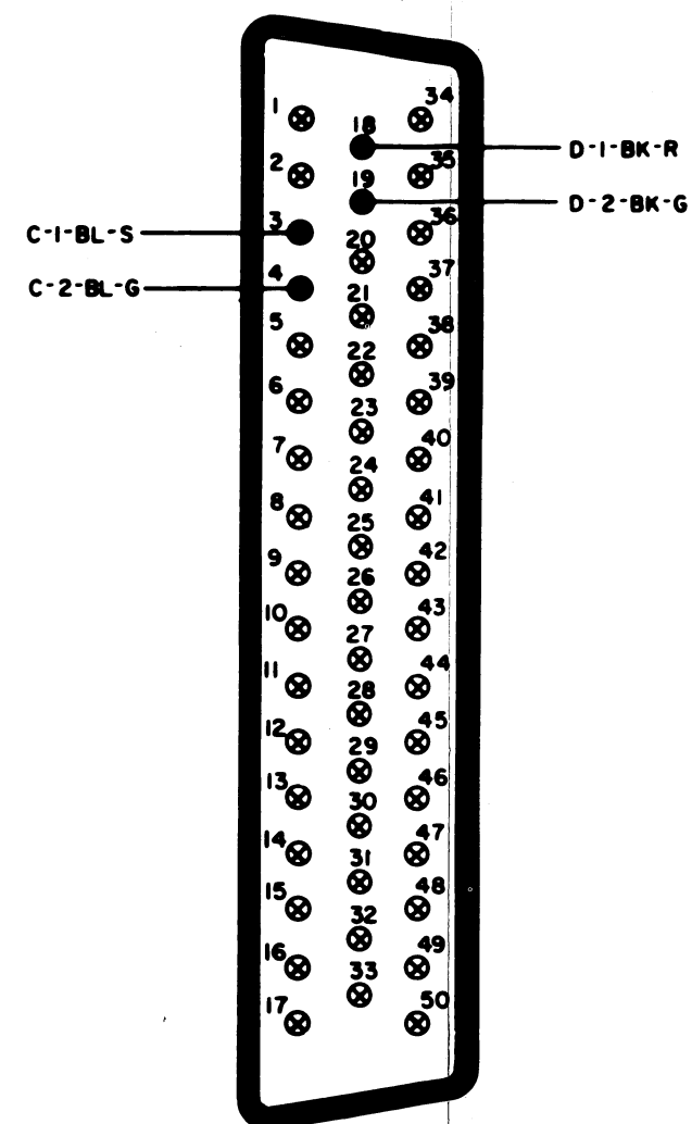
B REPERFORATOR CONNECTOR
